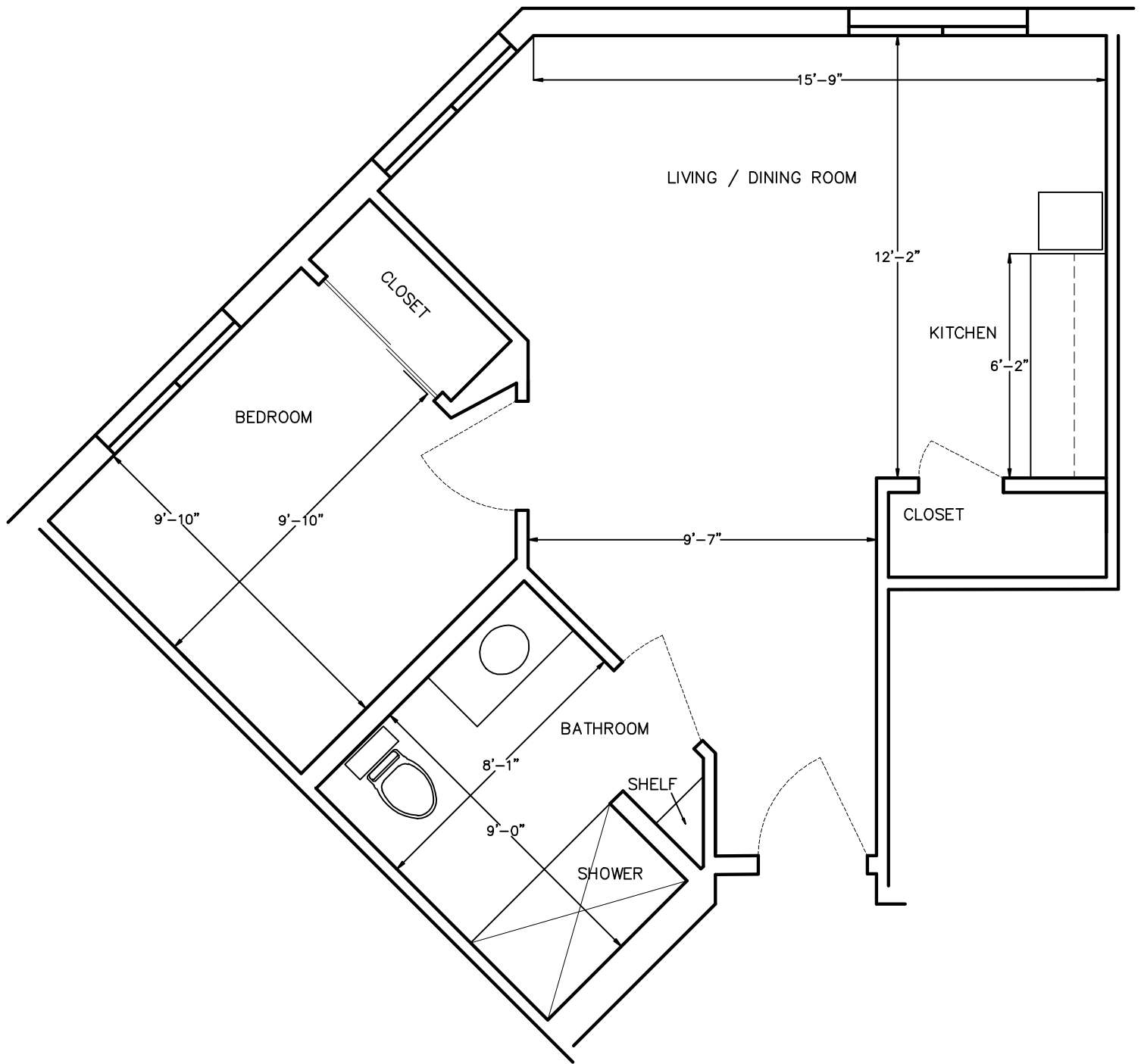
WYATT HOUSE SAMPLE FLOOR PLAN B
