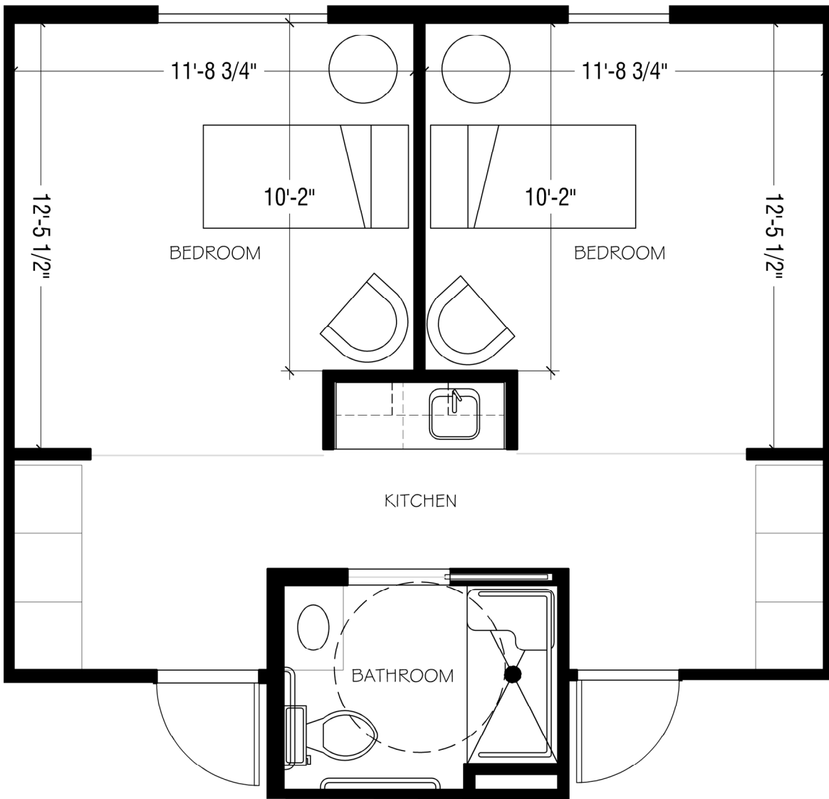
TWO BEDROOM - UNIT 418A - 474 sf
